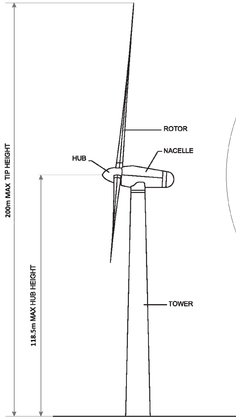
SIDE ELEVATION
