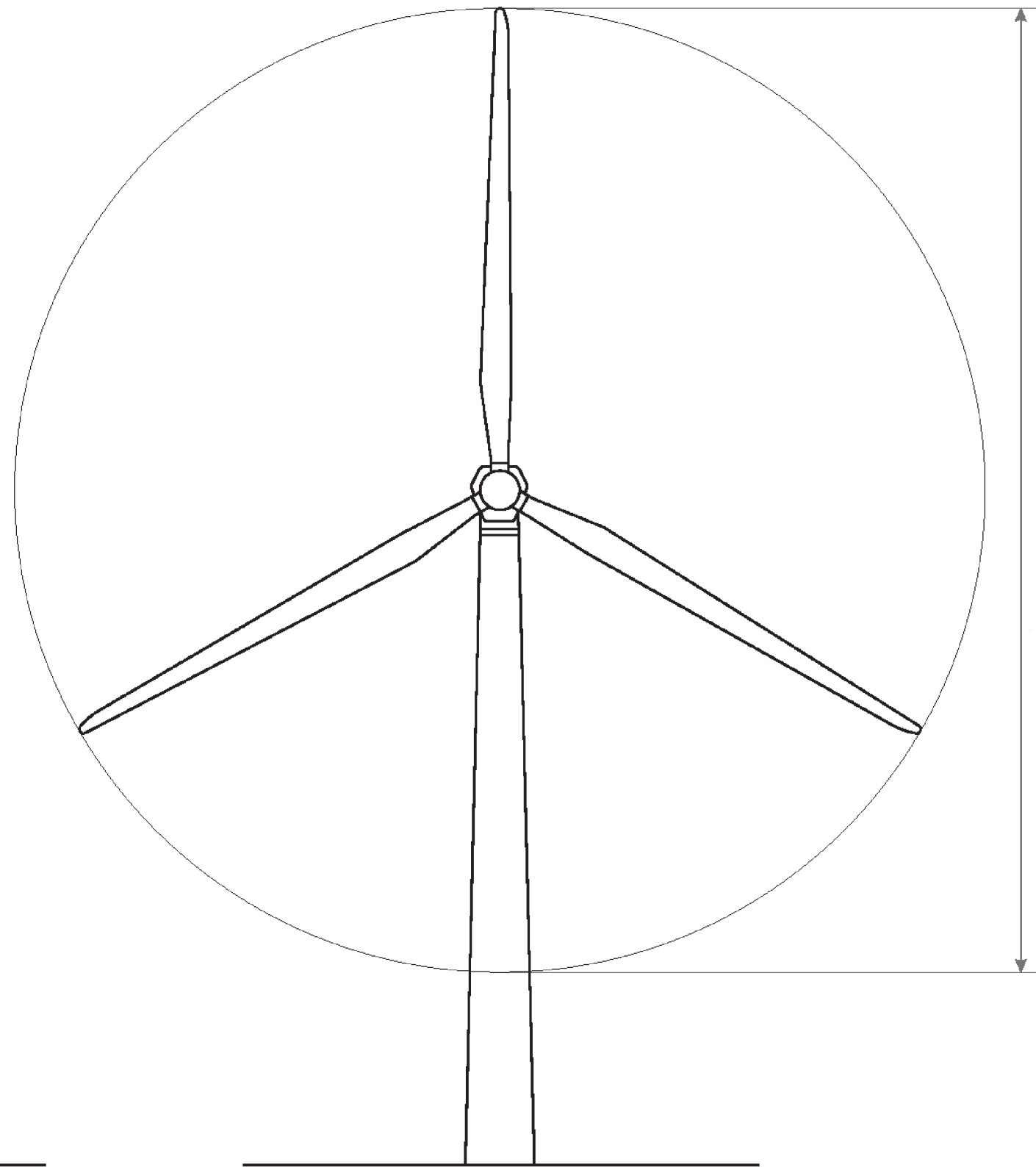
FRONT ELEVATION
